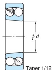
Tapered bore
