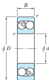
Cylindrical bore
