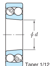
Tapered bore Taper 1/12
