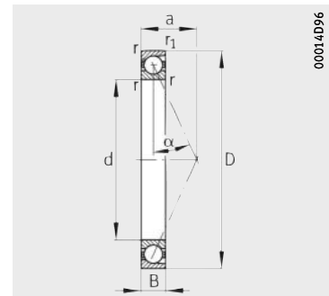
B719..-E, B70..-E, B72..-E \alpha = 25^\circ
